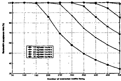
Figure 5. Bandwidth acceptance ratio for Greedy-penalty heuristic
