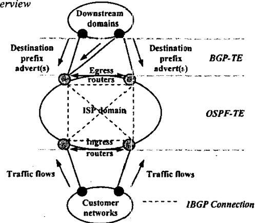
Figure 2. A general TE-enabled Internet architecture
