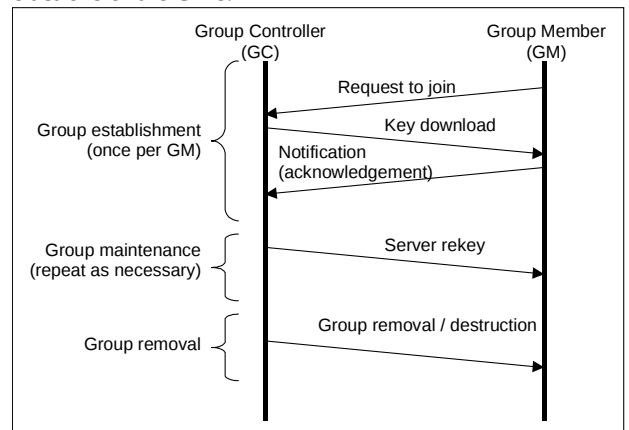
Fig. 3 GSAKMP message exchange
