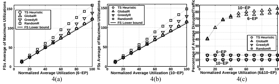
Figure 4. Performance evaluation for 6 and 10-EP topology
