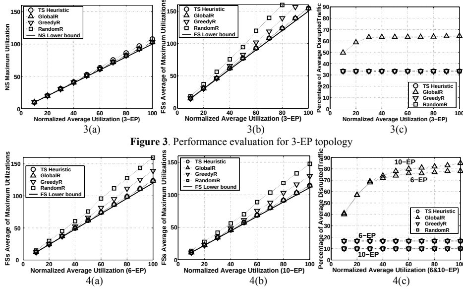
Figure 4. Performance evaluation for 6 and 10-EP topology
