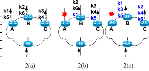
Figure 2 show the destination prefix assignment according to (a) OPTIMAL-AWARE HEURISTIC , (b) RANDOMR if EP A fails and (c) GLOBALR if EP A fails
