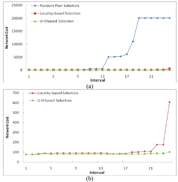
Figure 7. Network Cost performance
