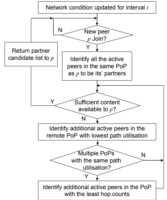
Figure 3. The U-H based peer selection algorithm
